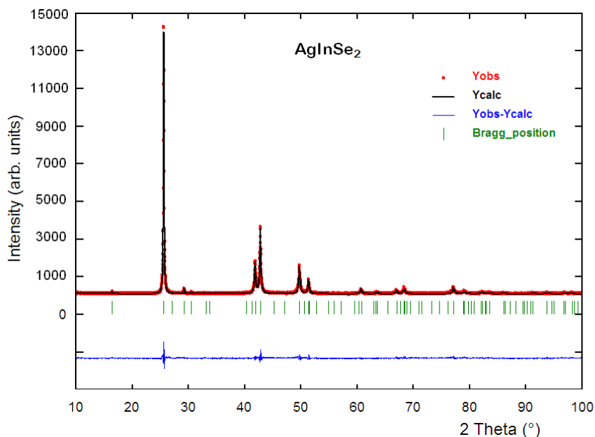
Figure 1. Final Rietveld refinement plot for \text{AgInSe}_2 . The lower trace is the difference curve between observed and calculated patterns. The Bragg reflections are indicated by vertical bars.
